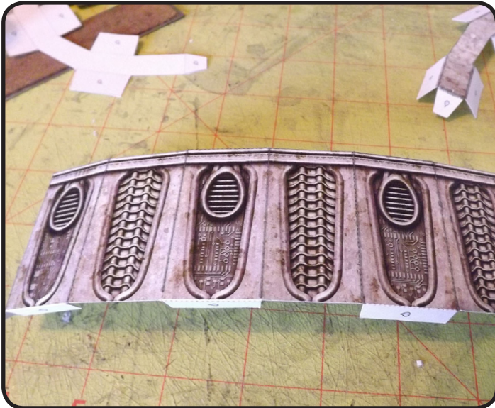
1: Cut, score and edge the individual wall pieces.
